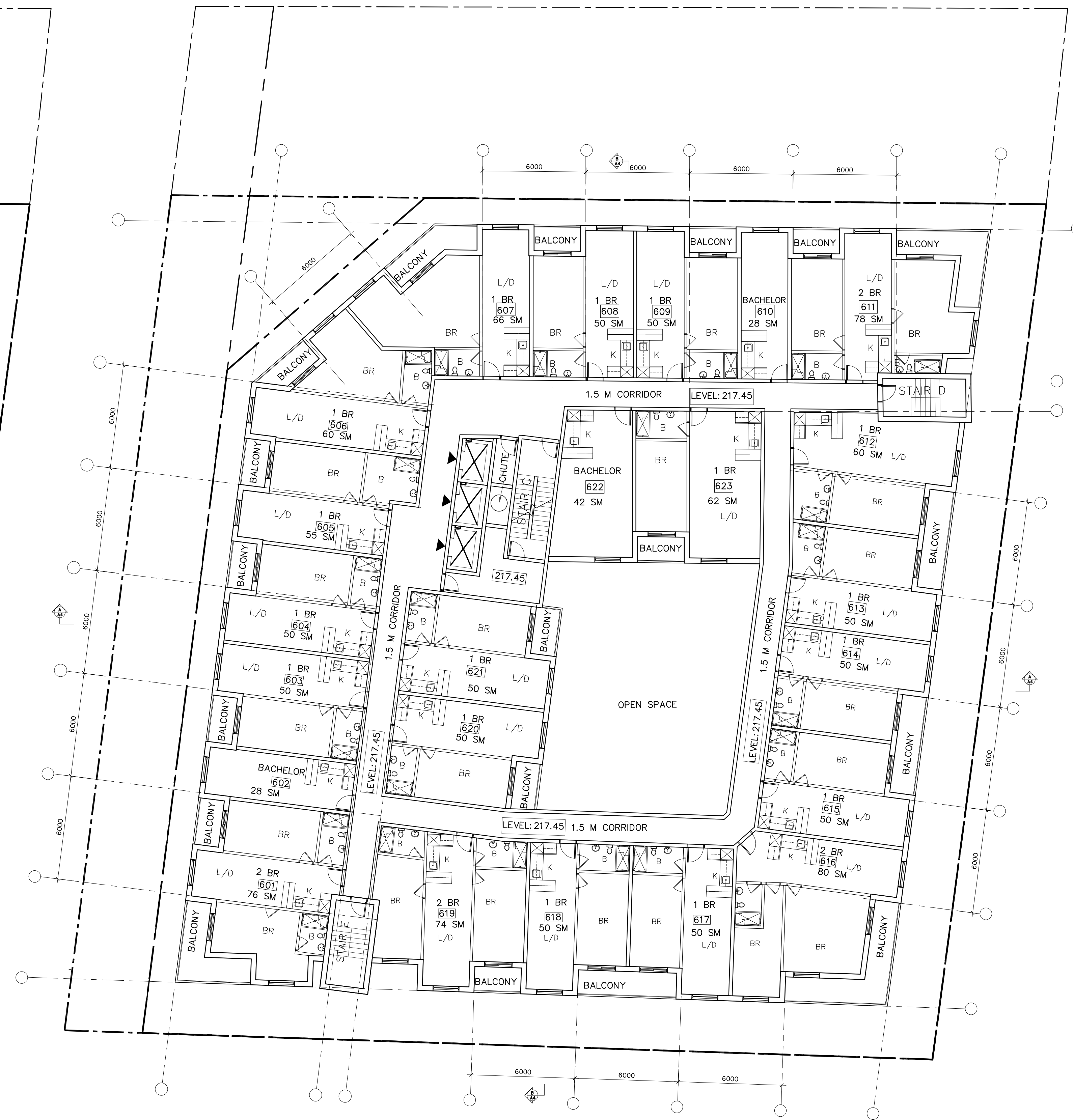
SIXTH FLOOR PLAN LEVEL 217.45 SCALE 1:150
